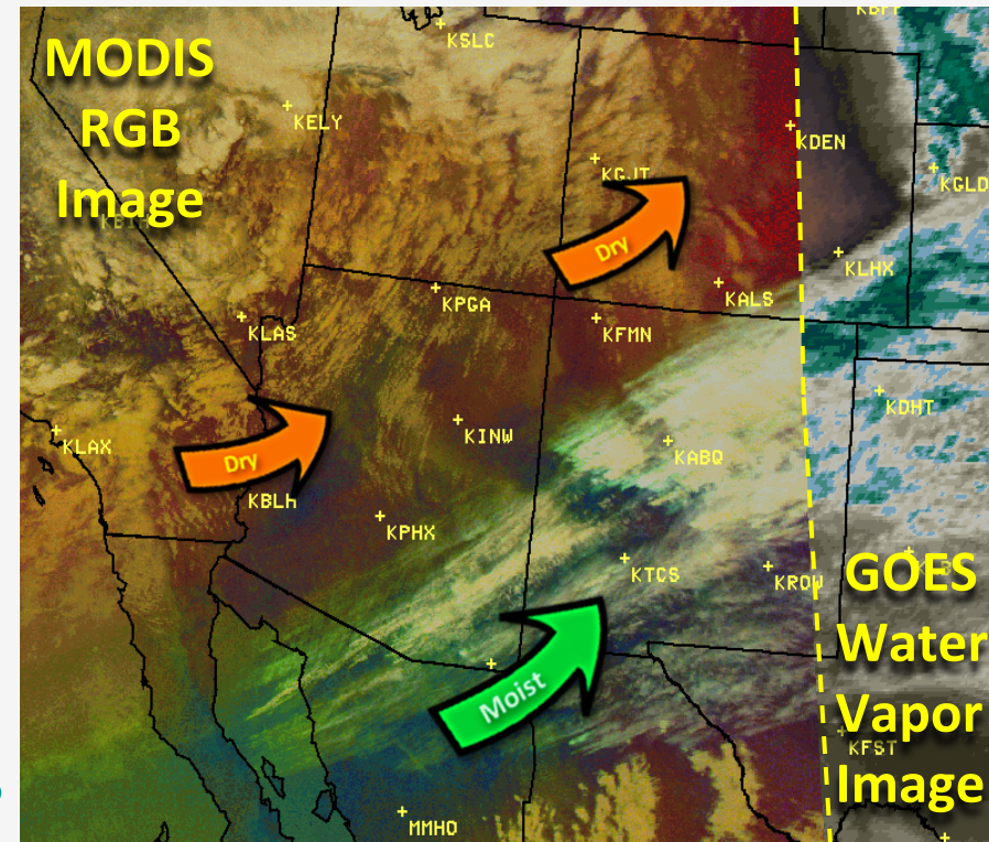
MODIS Airmass Red-Green-Blue (RGB) Image 200pm Friday, February 8, 2013
