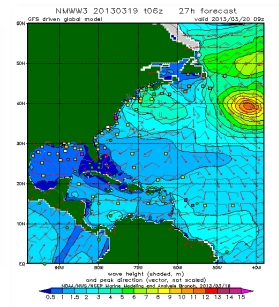
Wave Model Validation
