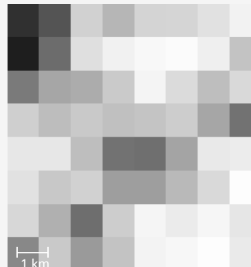
Satellite LSTs Resolution: 1km
