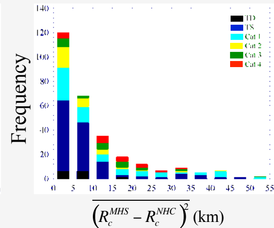
Cloudy Points
