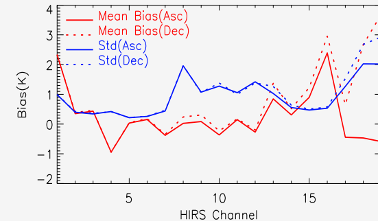
Metop-B
