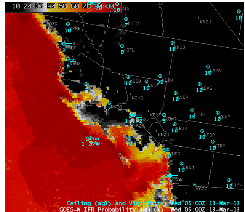
GOES-R IFR probabilities offshore Southern California
