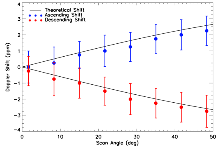
Doppler shift detected from CrIS observations
