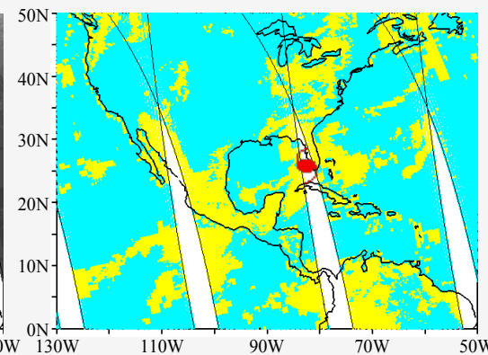
Cloudy Points
