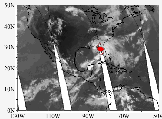
GOES-13 Ch4
